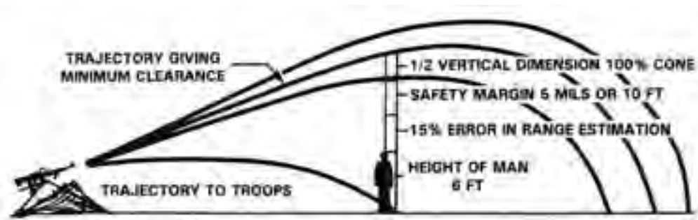
Figure 6-22. Components of Minimum Clearance.
