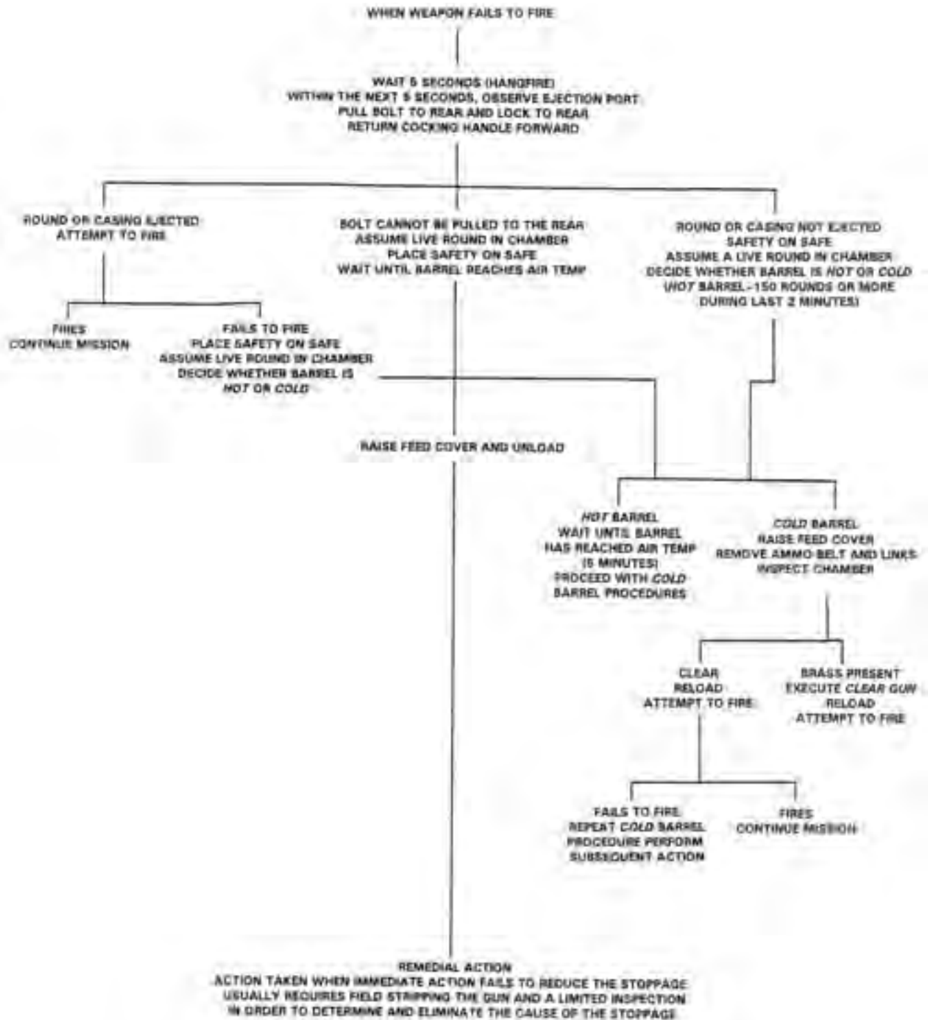
Figure 4-67. Immediate Action.
