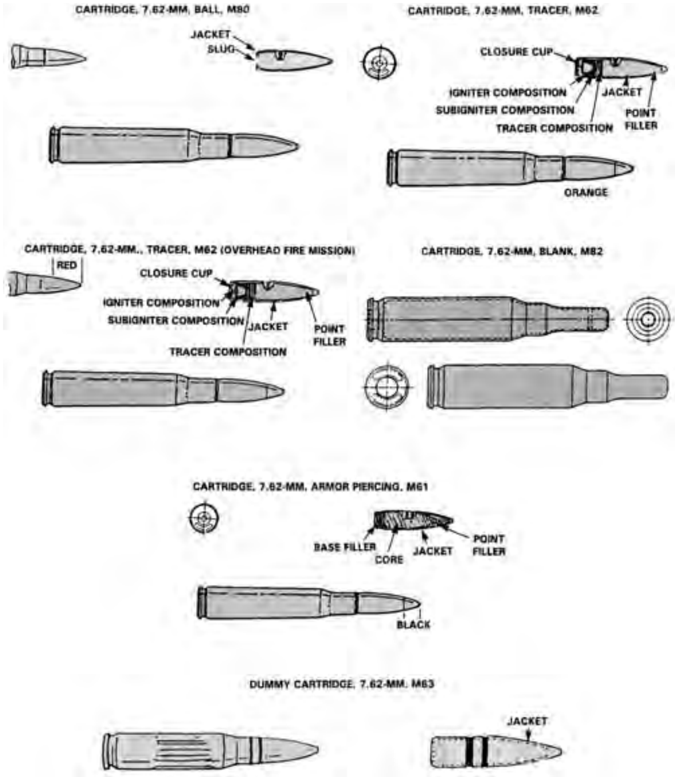
Figure 3-52. Ammunition for the M240G.
