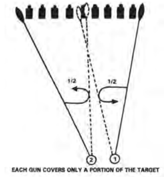
Figure 6-14. Traversing Method, Using a Squad of Guns. Target for Heavy Machine Gun More than 100 Mils in Width (Medium Machine Gun More than 50 Mils).
