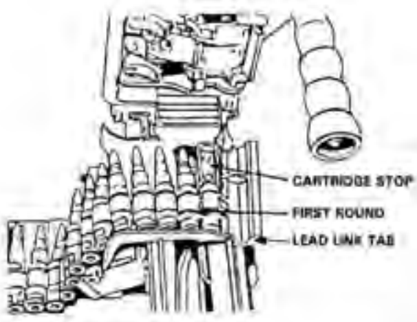
Figure 2-42. Cartridges in Metallic Belt.
