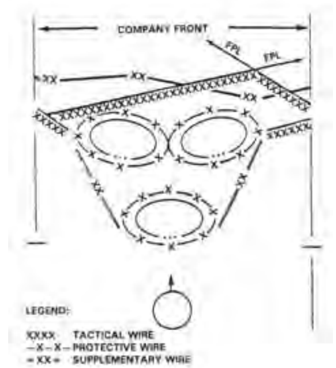
Figure G-2. Using Obstacles to Enhance the Effectiveness of the FPL.
