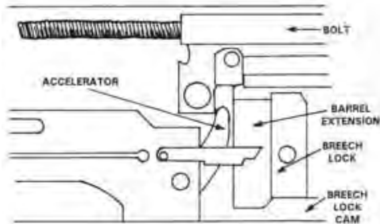
Figure 4-63. Locking.
