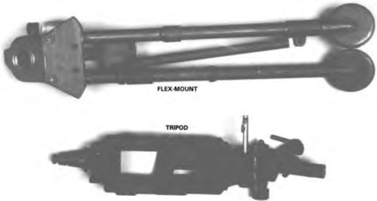
Figure 3-37. M12 Tripod and Flex-mount.
