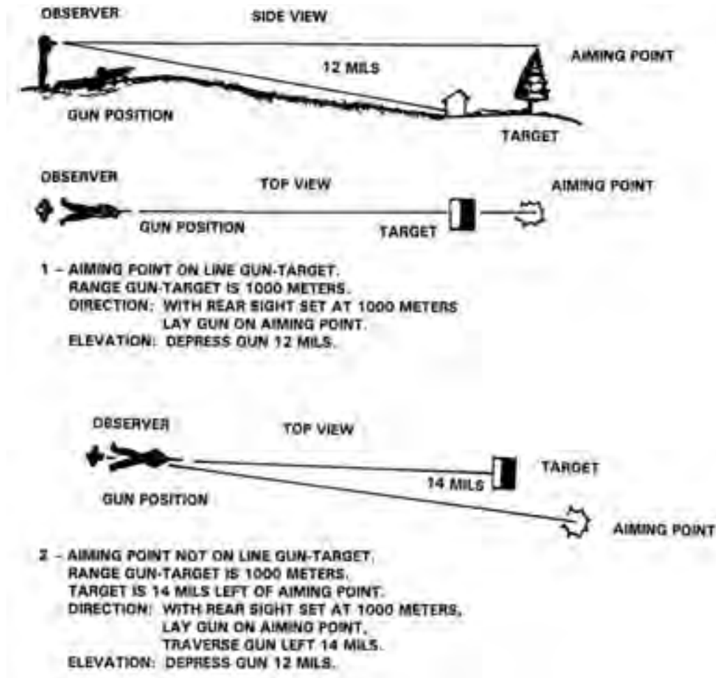
Figure 6-42. Aiming Point Method.
