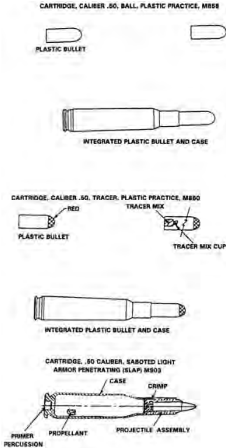
Figure 4-82. M2 .50 Cal Ammunition—Continued.
