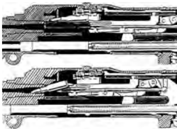
Figure 3-25. Chambering.
