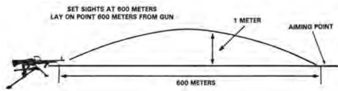
Figure 6-36. Method of Laying When the Ground is Level or Uniformly Sloping.
