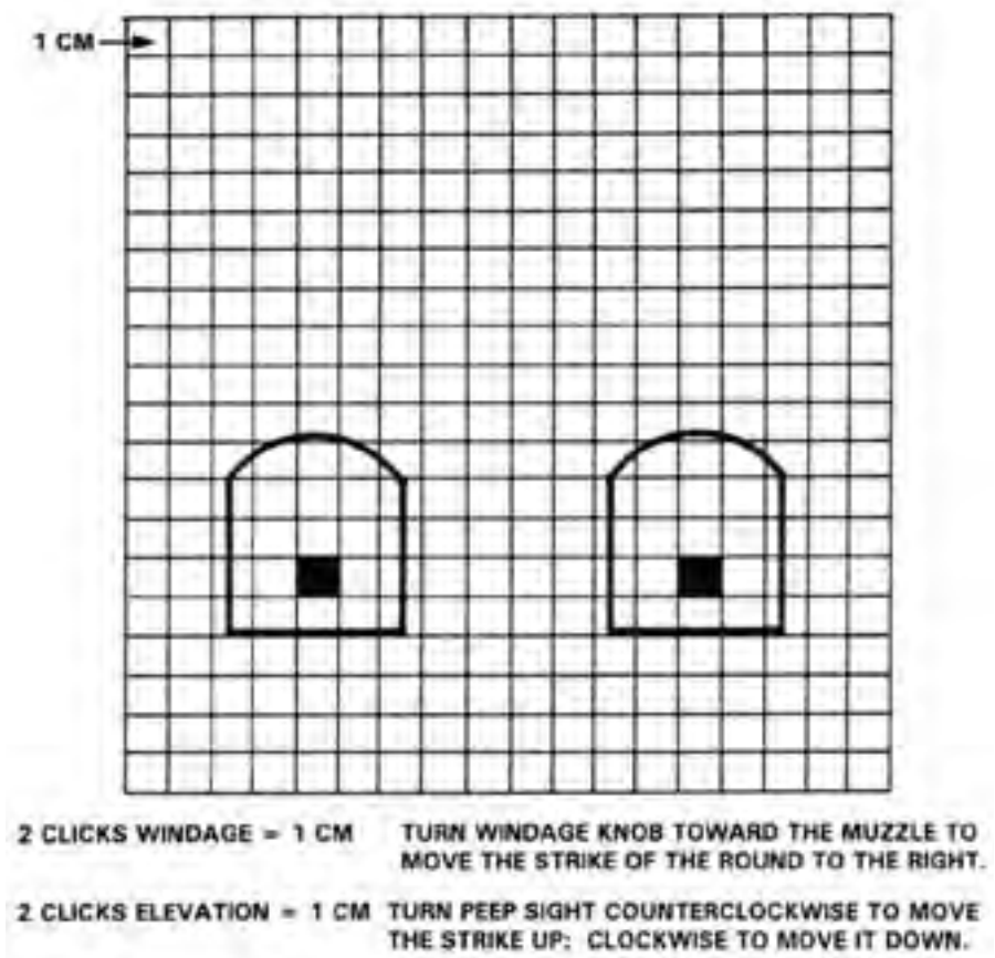
Figure 2-56. Grid Square Overlay.
