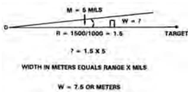
Figure 6-52. Estimating Mask Clearance.
