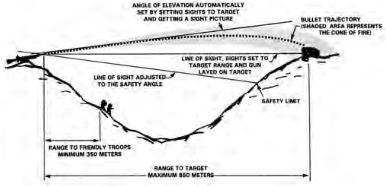
Figure 6-25. Gunner's Rule.
