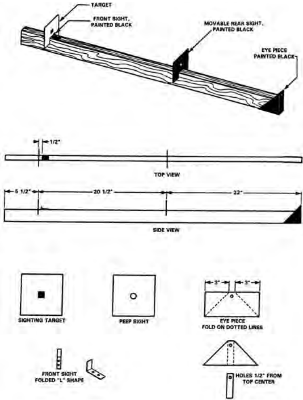
Figure 4-107. Sighting Bar.
