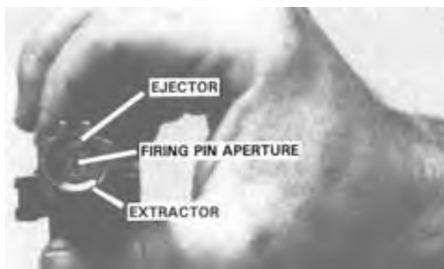
Figure 3-14. Bolt Face.
