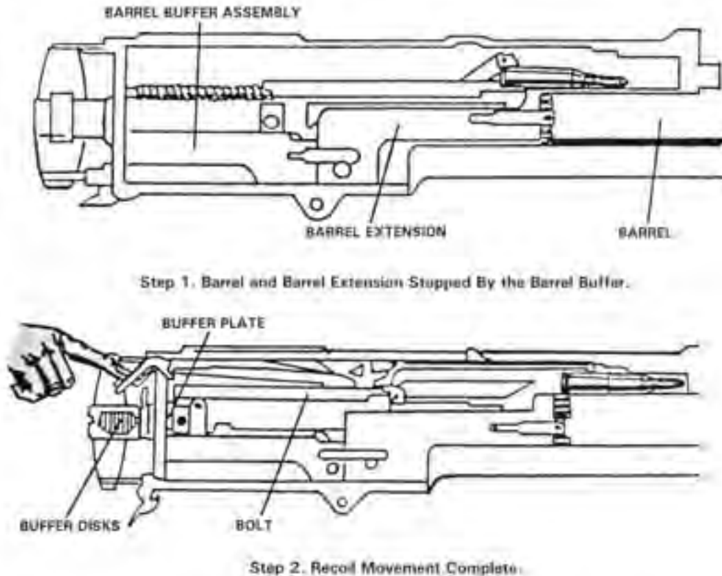
Figure 4-65. Unlocking.
