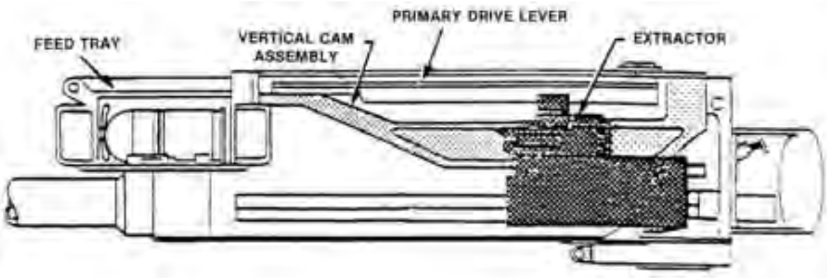
Figure 5-24. Round Positioned In Feeder, Bolt to Rear.
