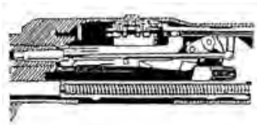
Figure 3-29. Unlocking.
