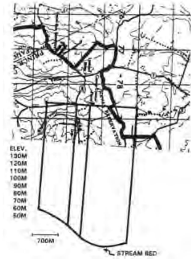
Figure 6-49. Sample Terrain Profile.
