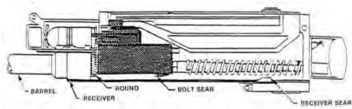
Figure 5-29. Chambering/Locking.
