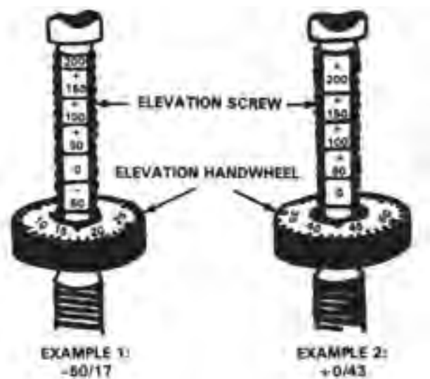
Figure 6-29. Elevation Reading.
