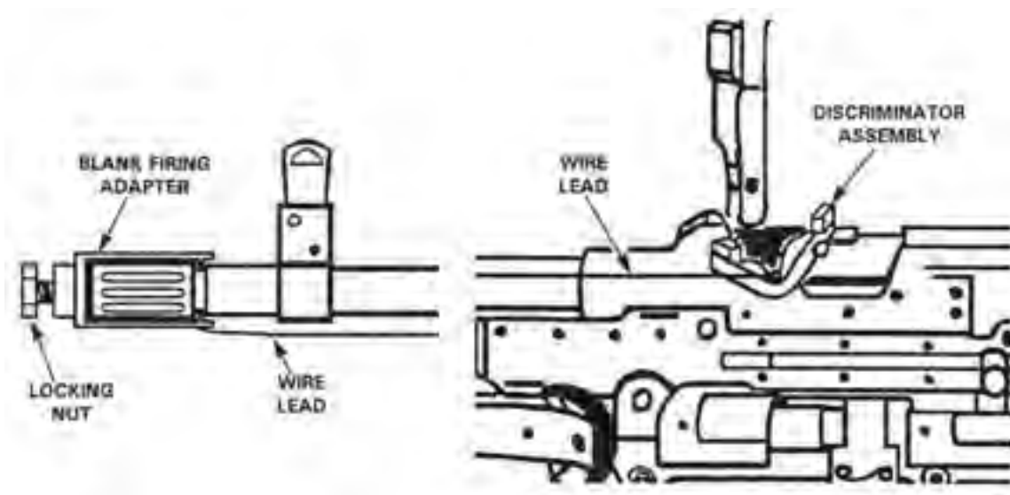
Figure 3-77. Installing the Blank Firing Adapter.
