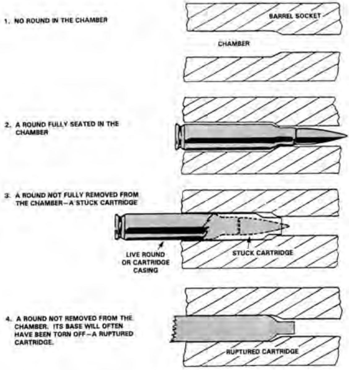
Figure 3-34. Chamber Condition During Immediate Action.
