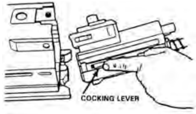
Figure 5-14. Inserting the Bolt and Backplate Assembly Into Receiver.
