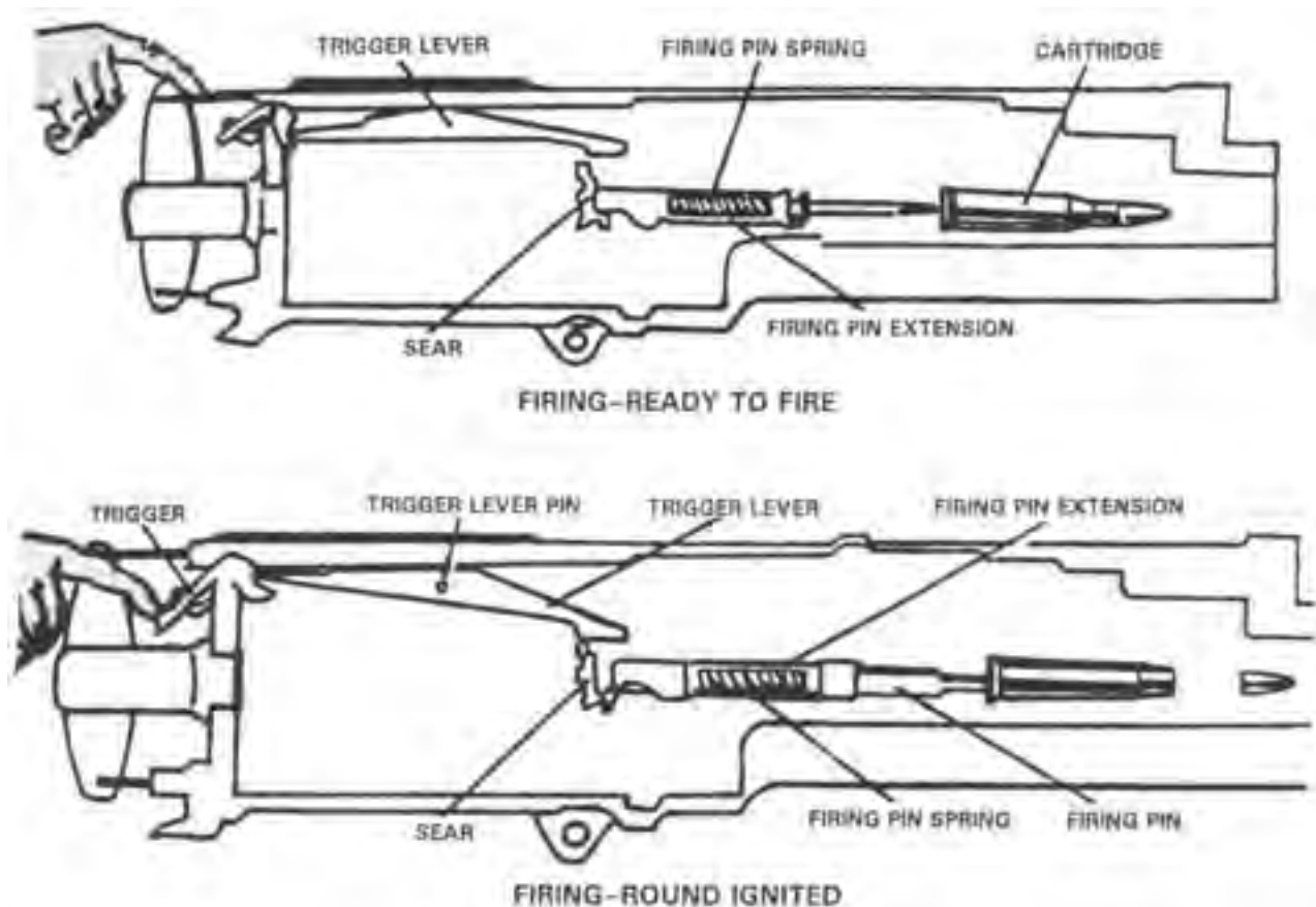
Figure 4-64. Firing.
