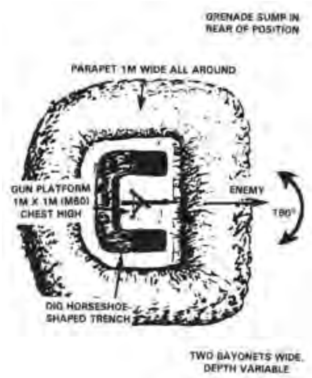
Figure 6-71. Horseshoe-Shaped Machine Gun Position.
