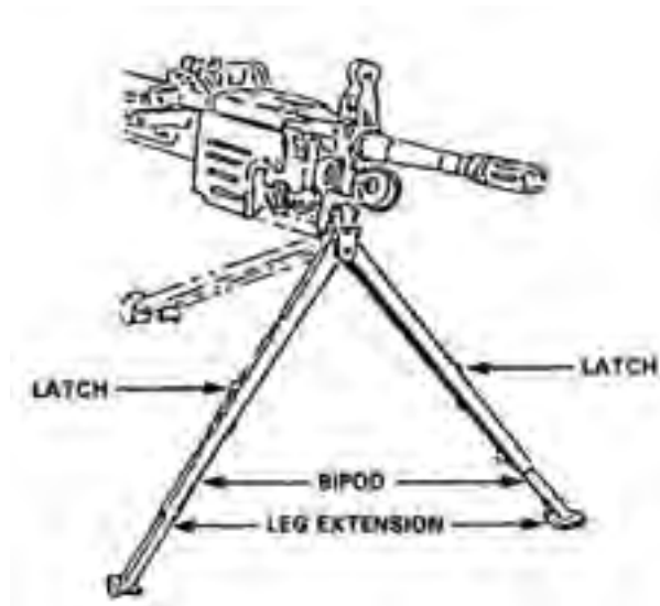
Figure 2-28. Lowering the Bipod.
