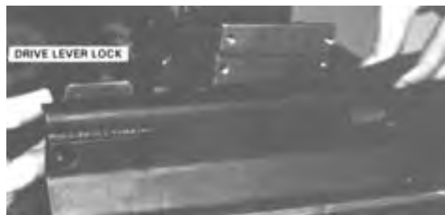
Figure 5-17. Retracting the Drive Lever Lock.
