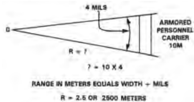
Figure 6-53. Estimating Range Using Known Width.
