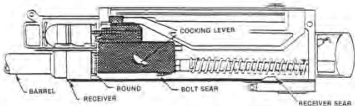
Figure 5-31. Extracting/Ejecting/Feeding/Cocking.
