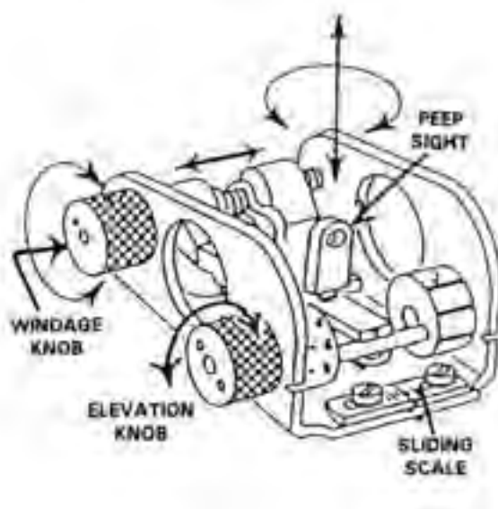
Figure 2-52. Sliding Scale on Sight.
