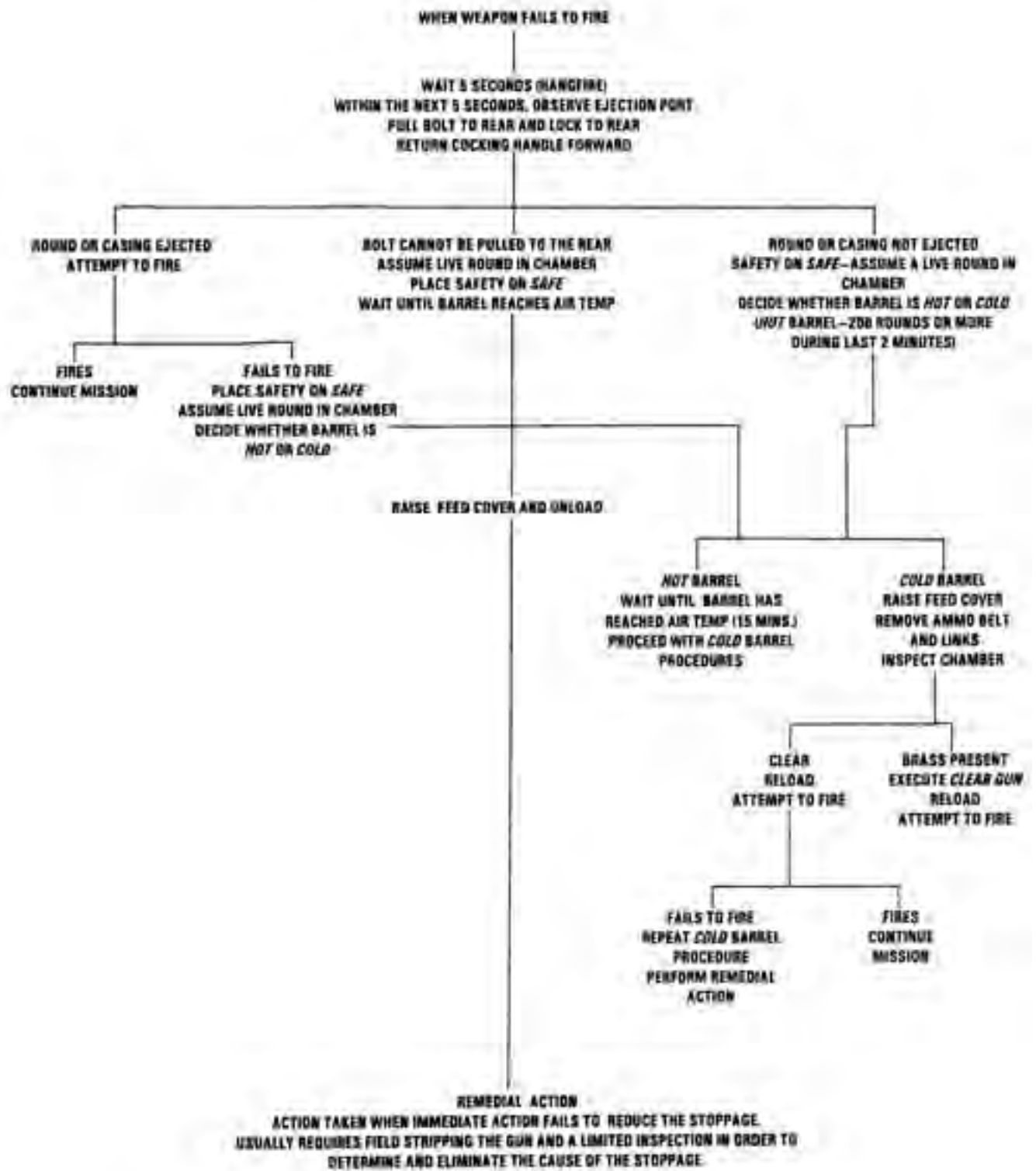
Figure 3-33. Immediate Action.
