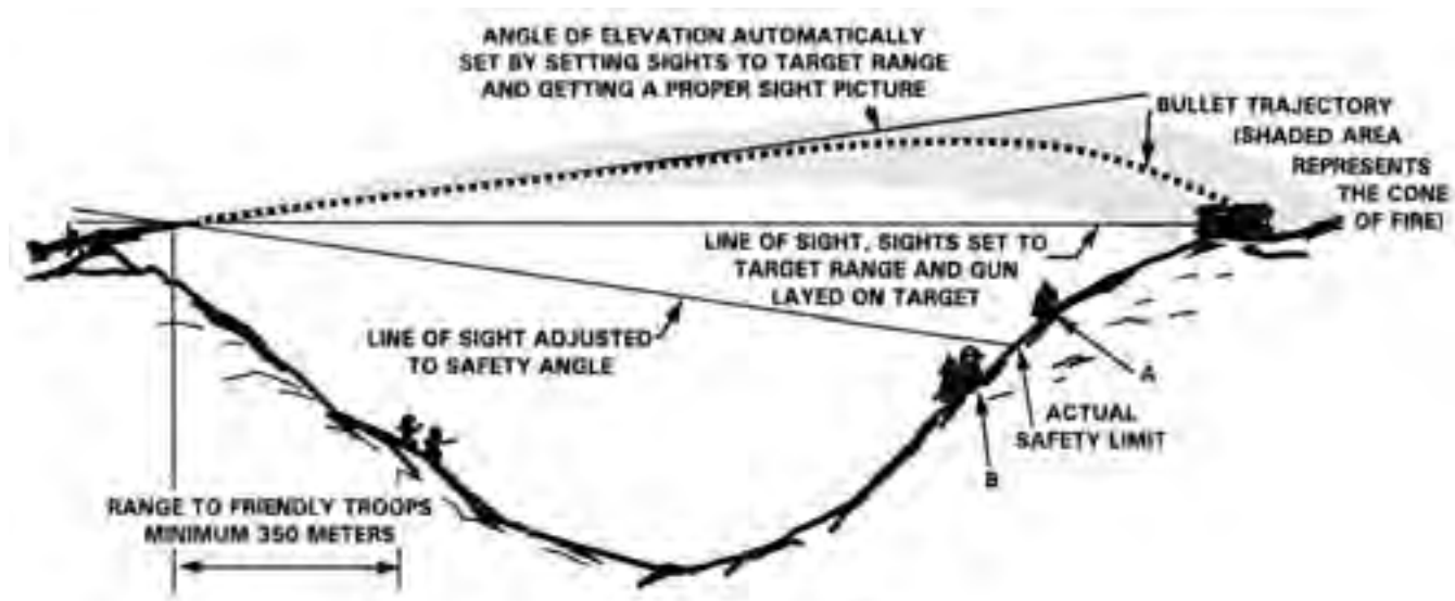
Figure 6-26. Leader's Rule.
