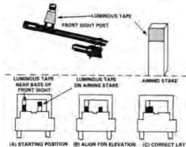
Figure 6-32. Field Expedient—Aiming Stake Method.
