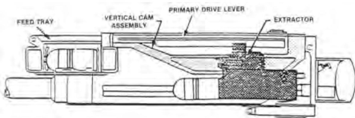
Figure 5-26. Round Cammed Down Onto Face of Bolt.
