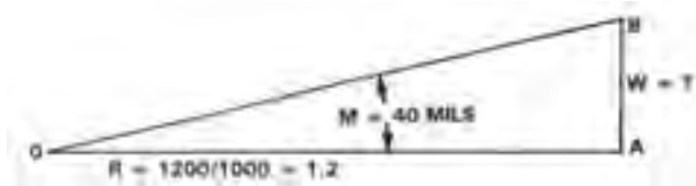
Figure 6-51. Estimating Distance Between Two Objects.
