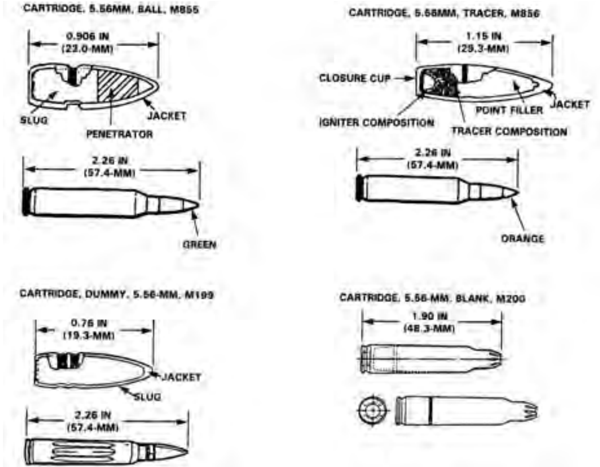
Figure 2-41. Cartridges for the SAW.
