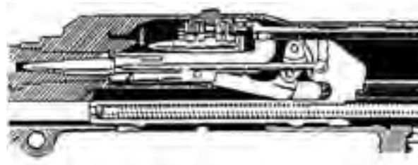
Figure 3-26. Locking.
