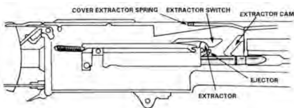
Figure 4-62. Chambering.
