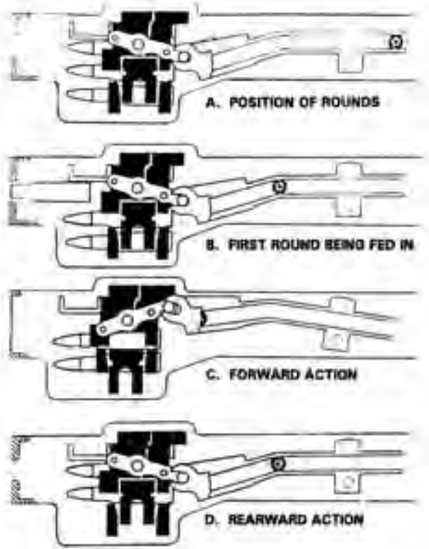
Figure 3-23. Feeding.
