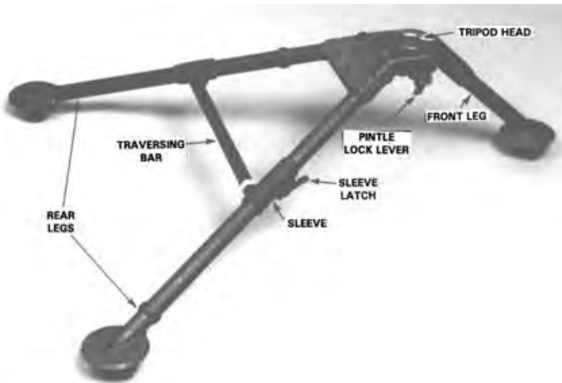
Figure 3-38. Tripod.
