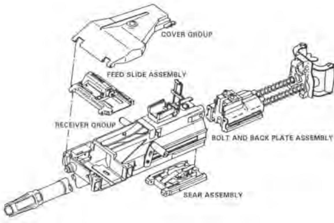
Figure 5-5. Five Main Groups, Exploded View.
