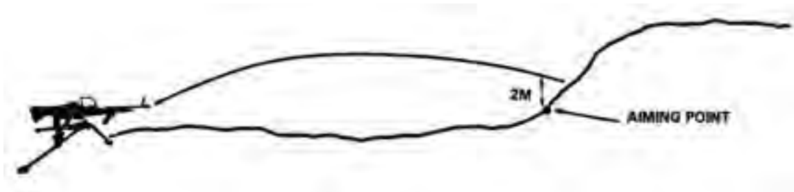
Figure 6-37. Method of Laying When There is a Break in the Uniform Slope (For Ranges Less Than 600 Meters).
